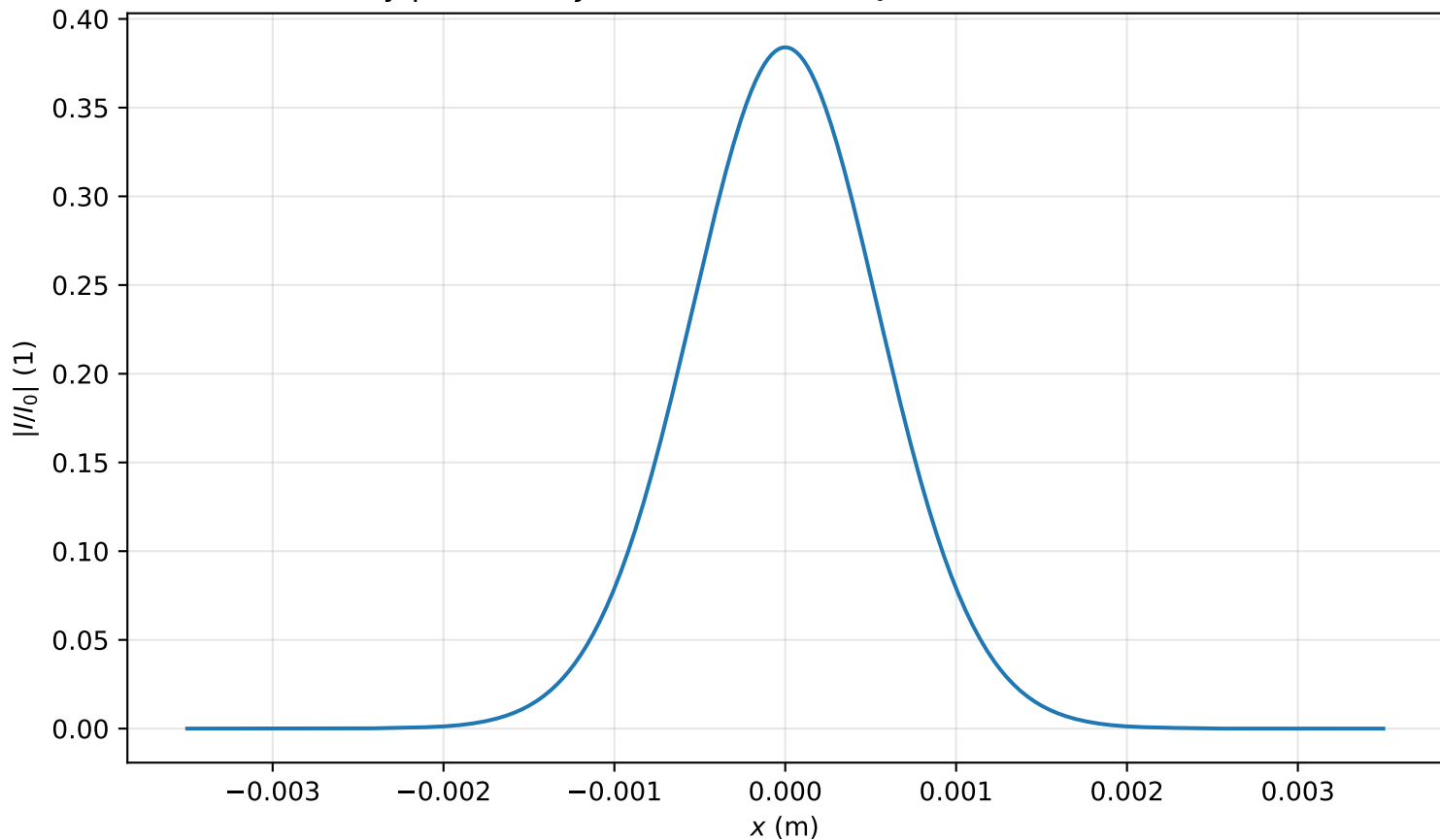
Intensity profile I(x, y = 0, z = 2.946m)/I_0 , P_{in}=0.2P_{cr} , artificial time
